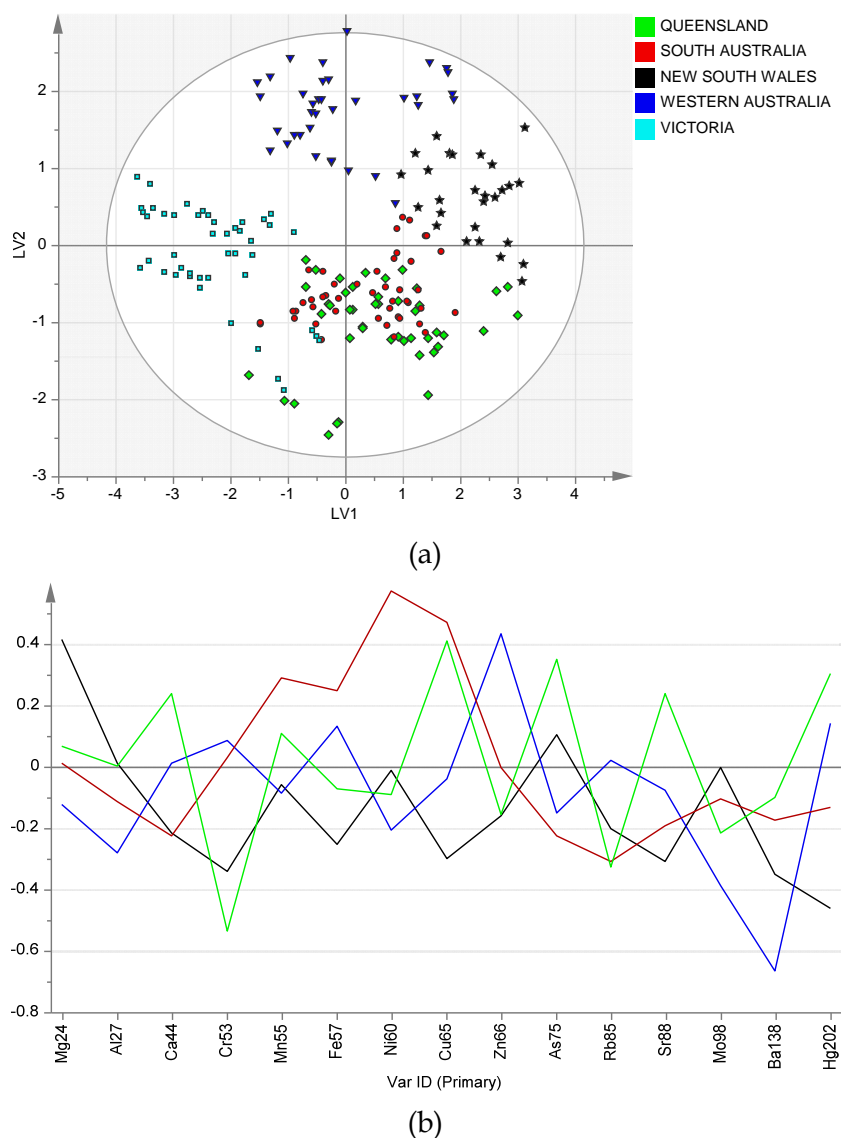
Figure 2 OPLS-DA of the LA-ICPMS data. (a) Scores plot LV1vs. LV2; Vic (light blue squares), NSW (black stars), WA (dark blue triangles), Qld (green diamonds), SA (red circles); (b) Corresponding loadings line plot. Black: LV1; Blue: LV2; Red: LV3; Green: LV4.
