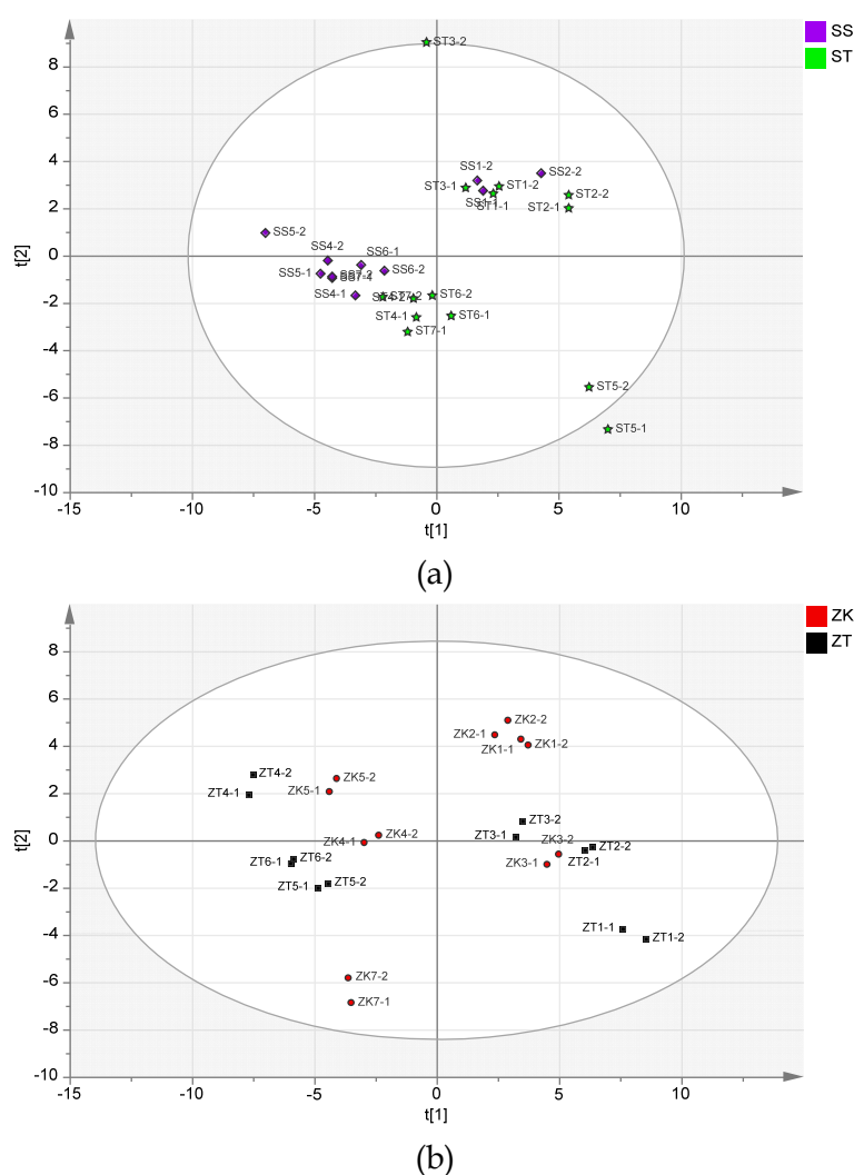
Figure 16 PCA scores plot of (a) "sanguineus" and (b) "zanzibariensis" specimens.
