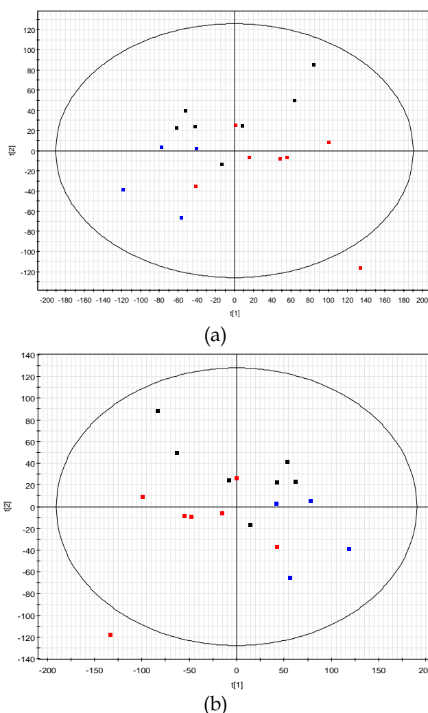
Figure 20 Analysis of the three “zibo 108” plants to assess for metabolome differences in the three morphologically different plants (black: tree 1; red: tree 2; blue: tree 3). (a) OPLS-DA scores plot (LV1 vs. LV2); (b) PLS-DA scores plot (LV1 vs. LV2).
