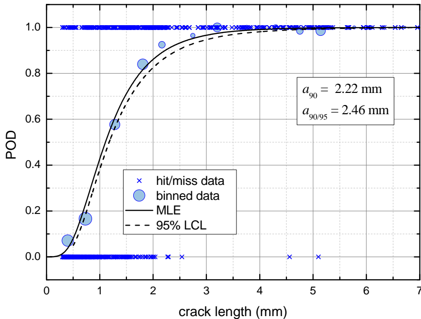
Figure 2 Notional POD curve for fluorescent MPT generated by pooling the hit/miss data from all six selected POD data sets. The total number of inspection results is n = 1329 .
